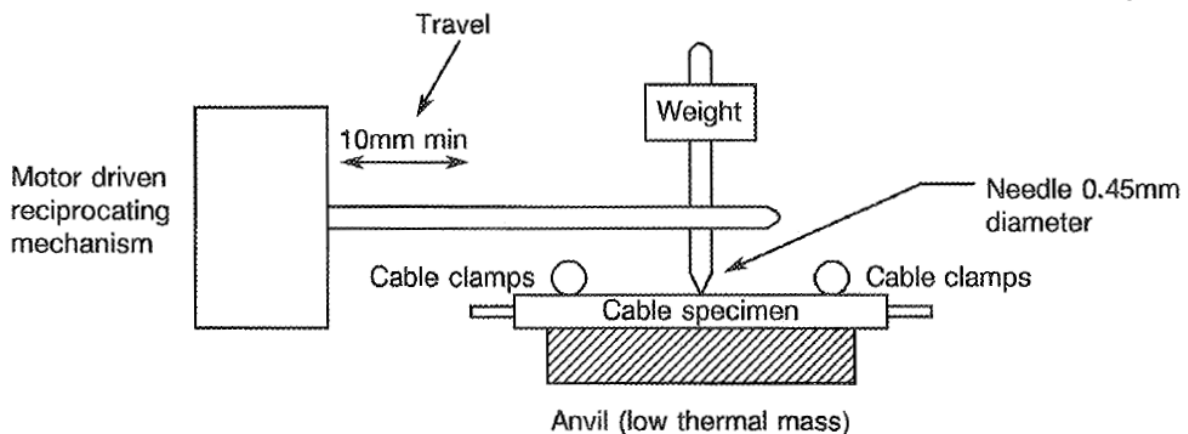
FIGURE I - ABRASION RESISTANCE TEST RIG
