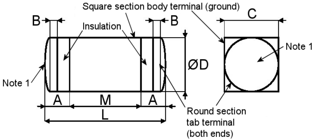
FIGURE 2 - PHYSICAL DIMENSIONS
