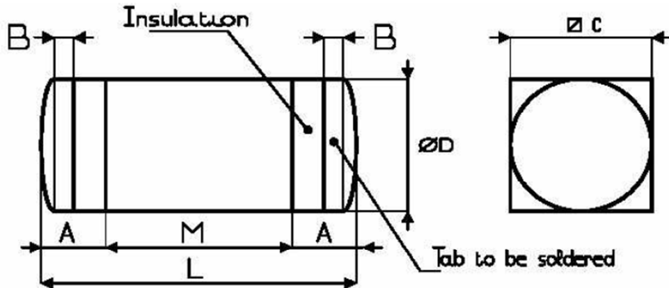
FIGURE 2 - PHYSICAL DIMENSIONS
