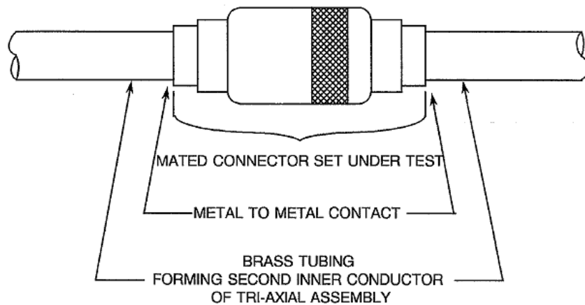
FIGURE II(a) - CONNECTOR ASSEMBLY FOR RF LEAKAGE TEST
