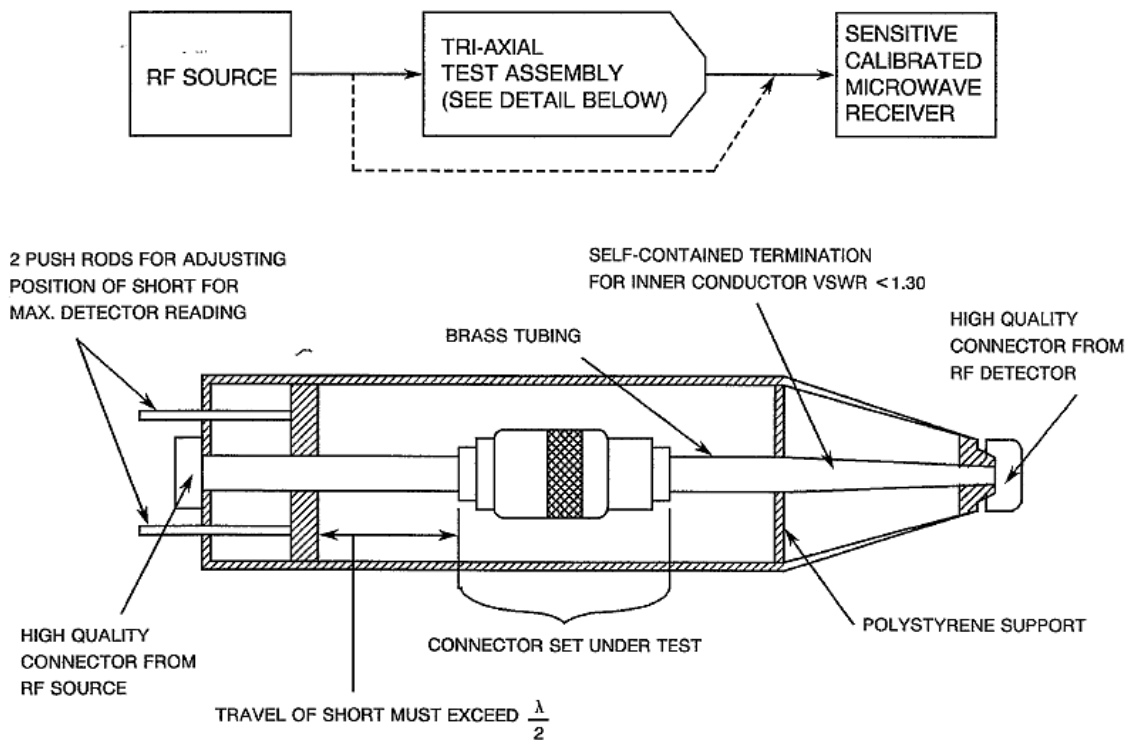
FIGURE II(b) - RF LEAKAGE TEST SET-UP
