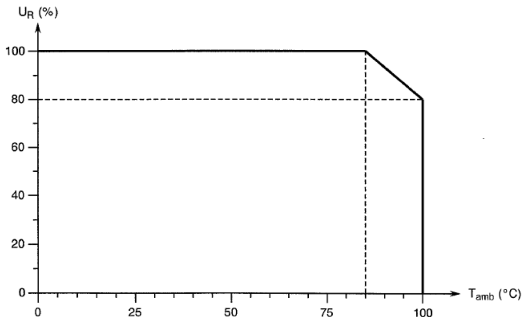
Rated Voltage versus Ambient Temperature
