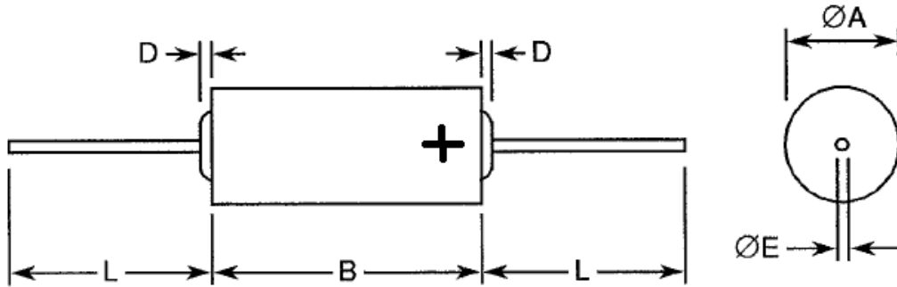
FIGURE 2 - PHYSICAL DIMENSIONS
