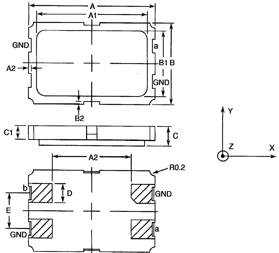
FIGURE 2 - PHYSICAL DIMENSIONS
