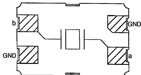
FIGURE 3 - FUNCTIONAL DIAGRAM
