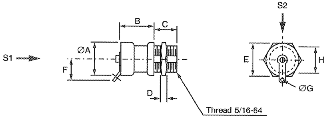
FIGURE 2(a) - VARIANT 01, LUG PANEL MOUNT
