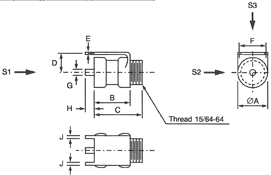
S1, S2, S3 – Vibration and Shock axes
