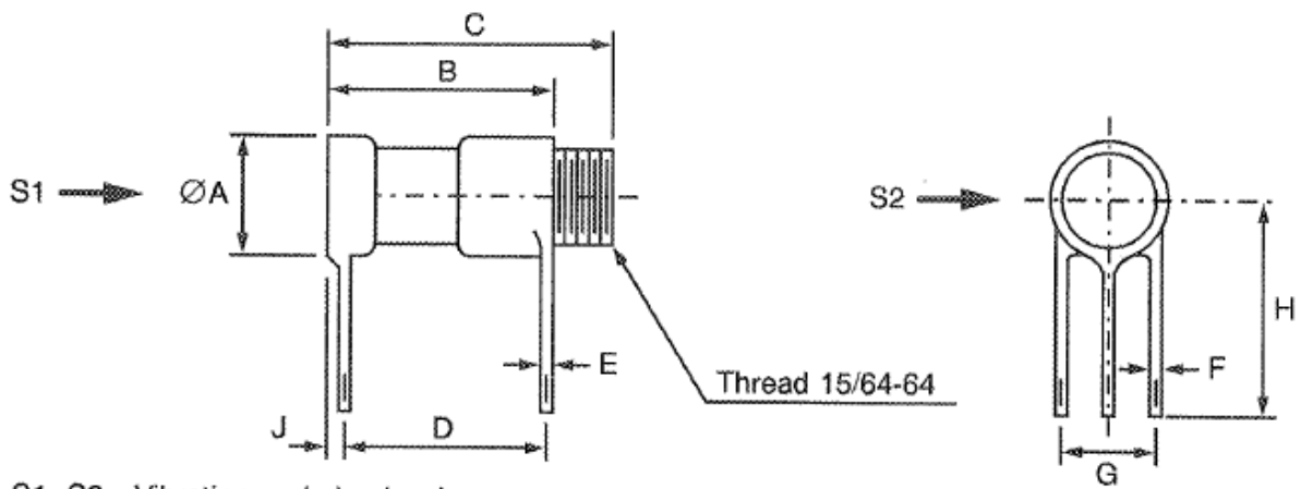
FIGURE 2(c) - VARIANT 03, PCB MOUNT
