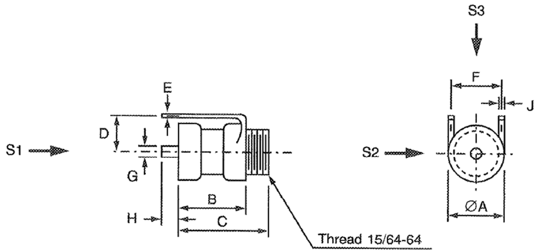
FIGURE 2(e) - VARIANT 05, SPECIAL VERTICAL MOUNT
