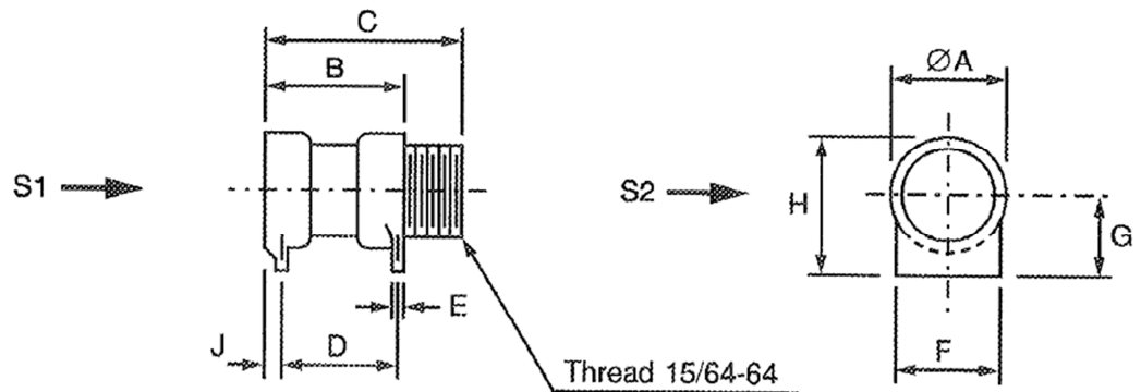
FIGURE 2(f) - VARIANT 06, STRIP LINE MOUNT
