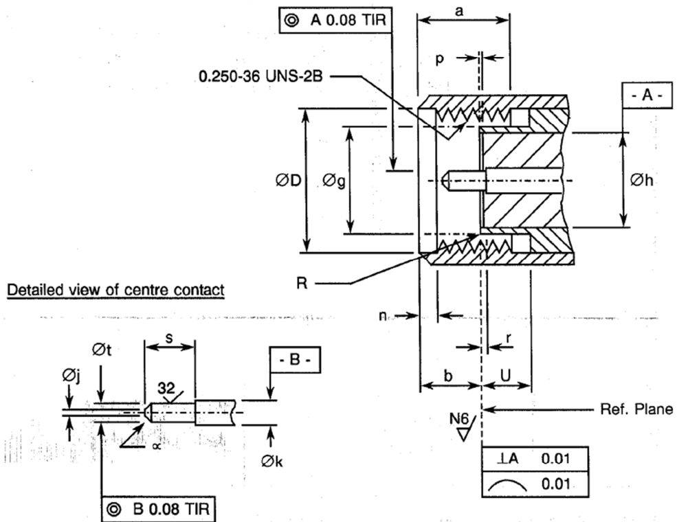
FIGURE 3 - STANDARD TEST CONNECTOR INTERFACE (CONTINUED) - MALE CONTACT
