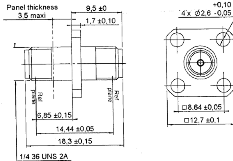
VARIANT 10 - STRAIGHT FLANGE ADAPTOR, FEMALE - FEMALE
