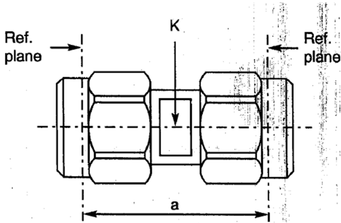
VARIANT 11 - STRAIGHT ADAPTOR, MALE - MALE
