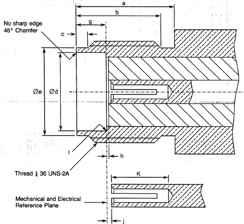
FIGURE 2(a) - CONNECTOR INTERFACE (CONTINUED) - FEMALE CONTACT
