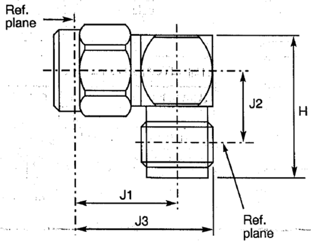
VARIANT 05 – ELBOW ADAPTOR, MALE - FEMALE
