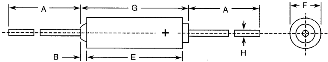
FIGURE 2 - PHYSICAL DIMENSIONS
