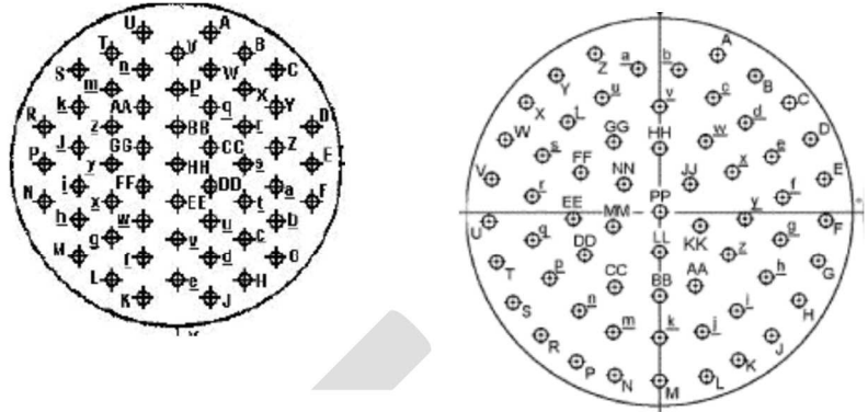
FIGURE 2(b) – SPECIAL CONTACT ARRANGEMENTS – FRONT VIEW MALE INSERT
