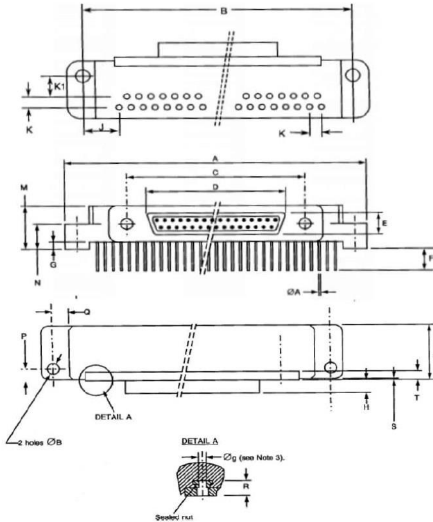
FIGURE 2.2B - CONNECTORS TYPE - FR136 RECEPTACLE FEMALE CONTACTS
