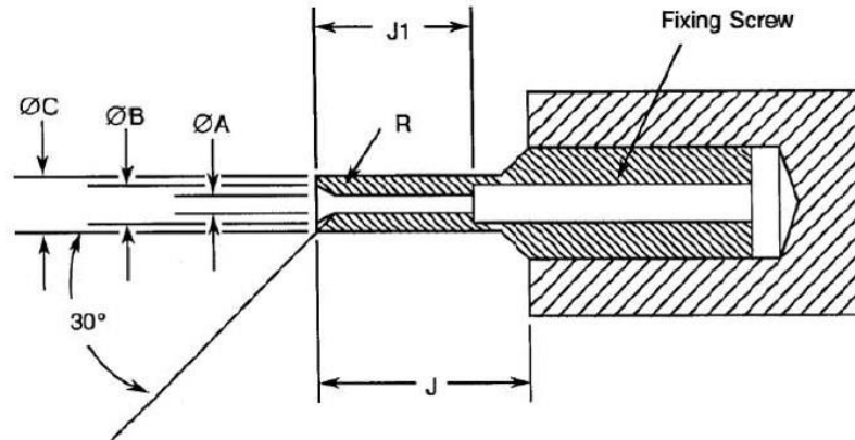
FIGURE 4 - GAUGE FIXTURE
