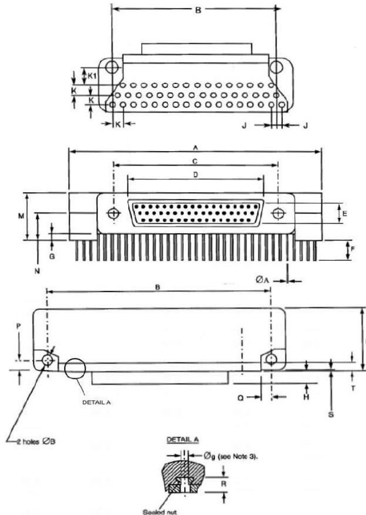
FIGURE 2.2D - CONNECTORS TYPE - FR136 RECEPTACLE FEMALE CONTACTS
