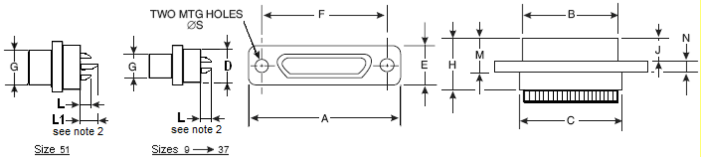
FIGURE 2.1C CONNECTORS TYPE FR164 - PLUG MALE CONTACTS
