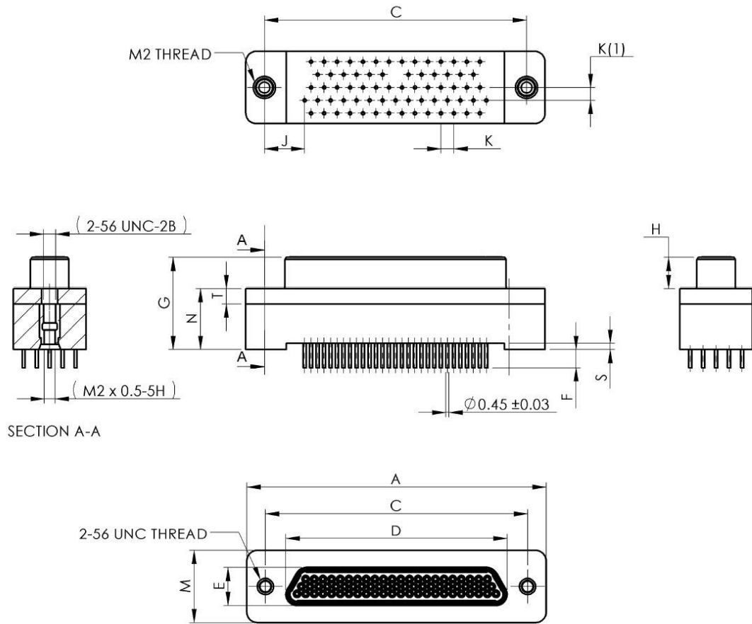
FIGURE 2.2U - CONNECTORS TYPE – GMR7580 RECEPTACLE FEMALE CONTACTS
