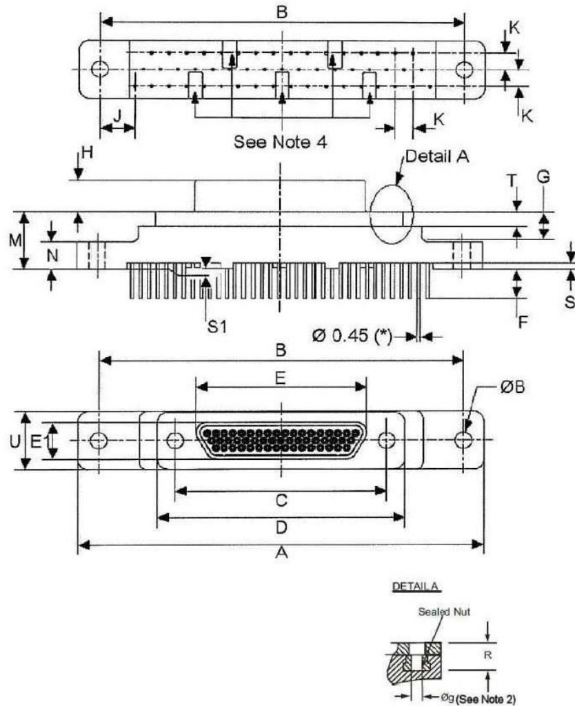
FIGURE 2.2J - CONNECTORS TYPE - FR139 RECEPTACLE FEMALE CONTACTS - SIZE 51
