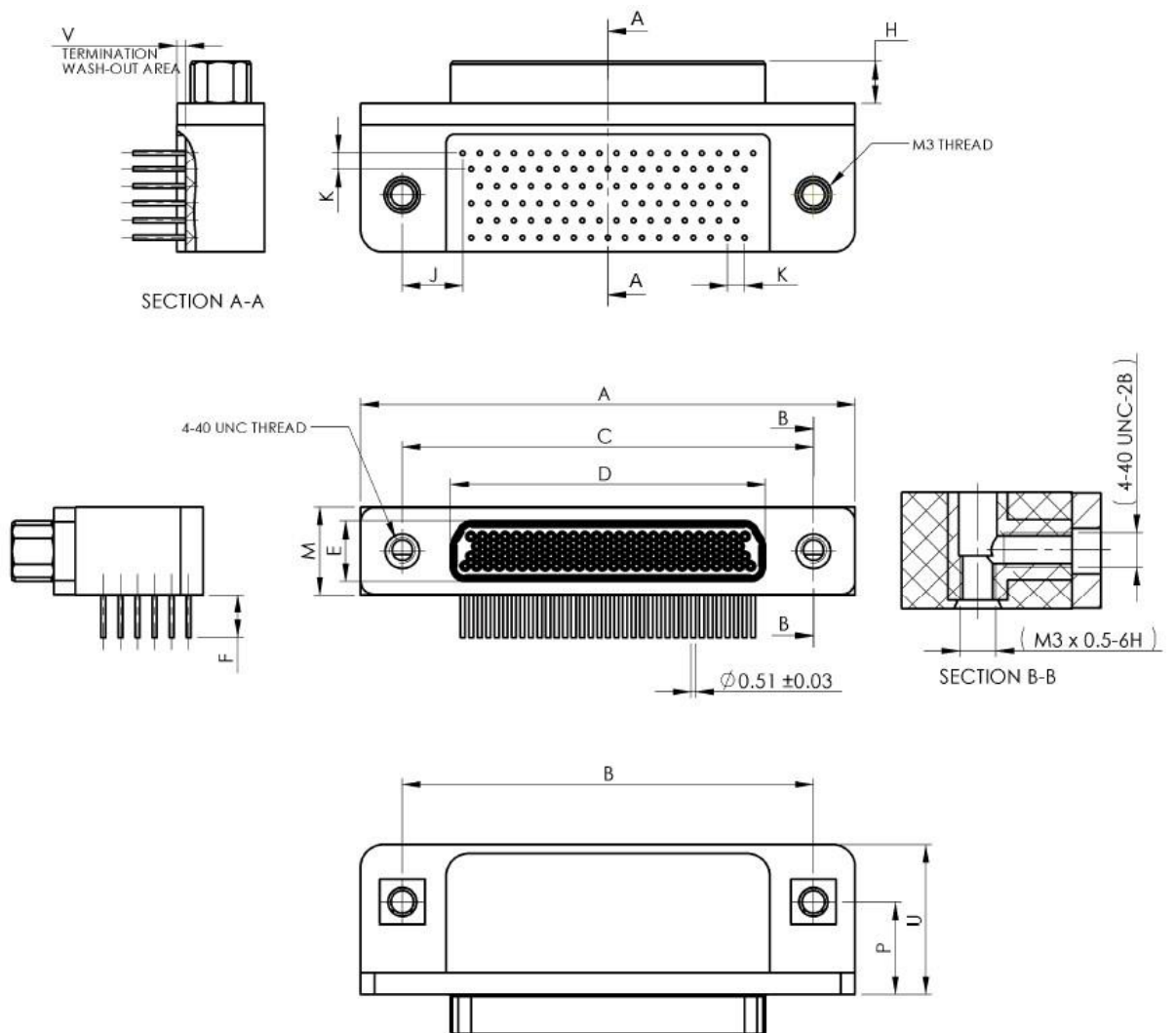
FIGURE 2.2P - CONNECTORS TYPE – GMR7590 PLUG MALE CONTACTS
