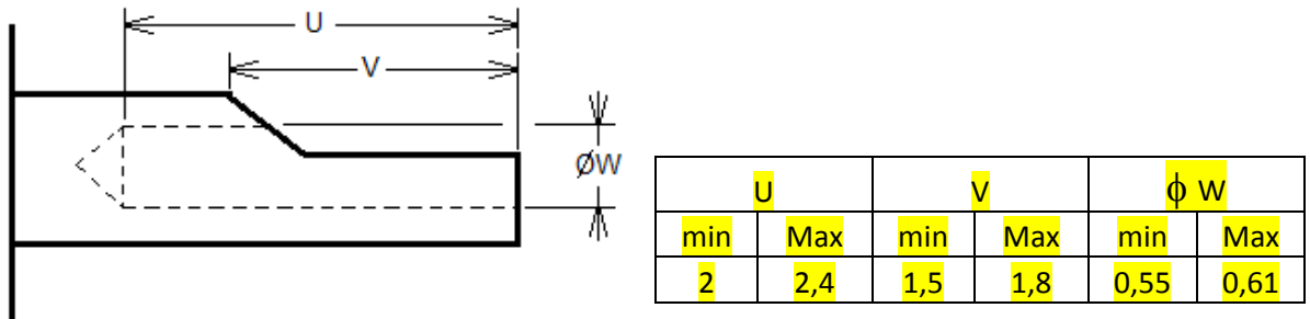
FIGURE 2.6 – SOLDER BUCKET
