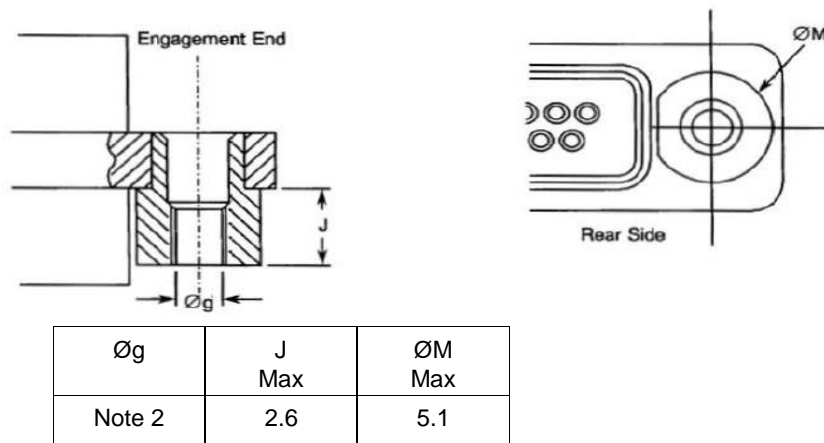
FIGURE 2.8 - CAPTIVE NUT
