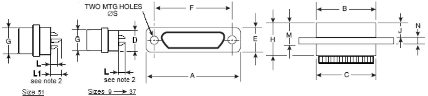
FIGURE 2.1D CONNECTORS TYPE FR164 - RECEPTACLE FEMALE CONTACTS
