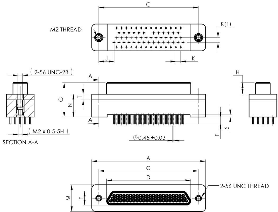
FIGURE 2.2T - CONNECTORS TYPE – GMR7580 PLUG MALE CONTACTS
