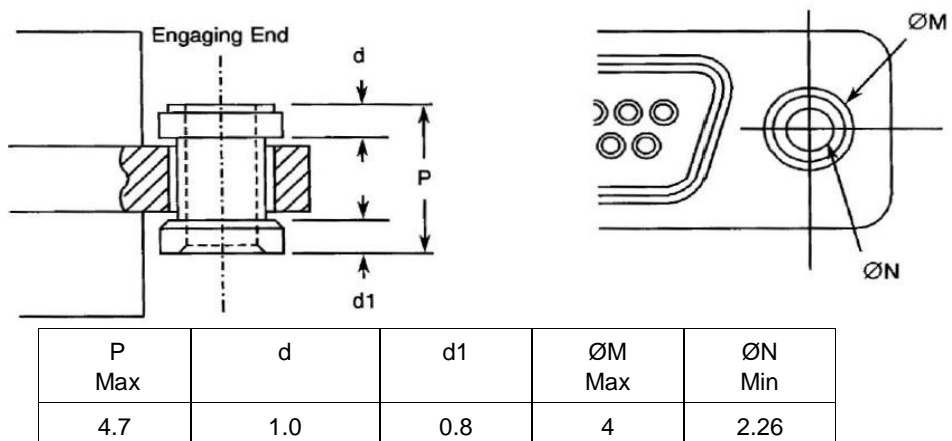
FIGURE 2.7 - FLOATING MOUNT
