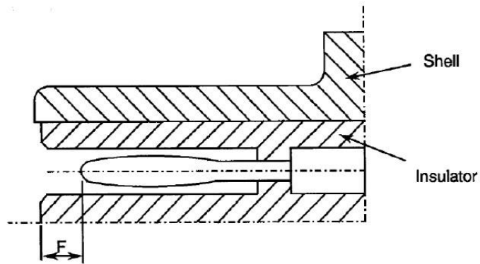
FIGURE 2.3.2 - PLUG MALE CONTACT
