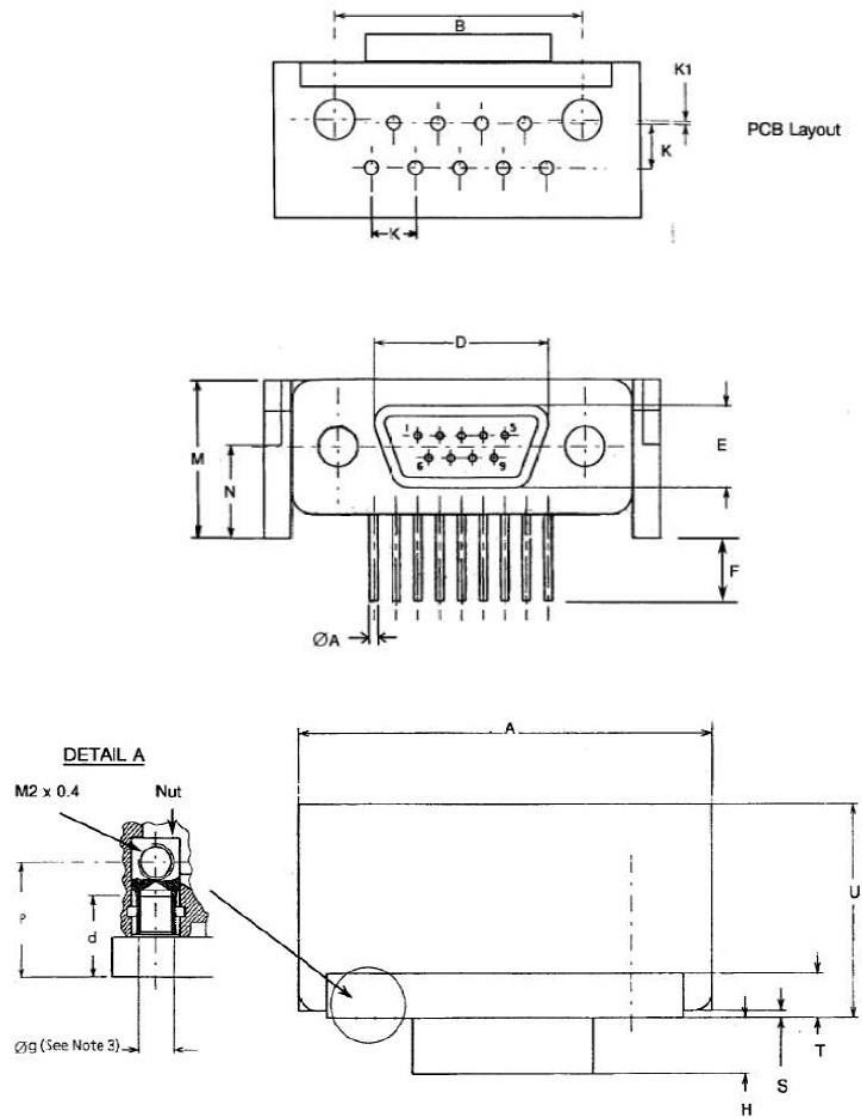
FIGURE 2.2F - CONNECTORS TYPE - FR136A RECEPTACLE FEMALE CONTACTS
