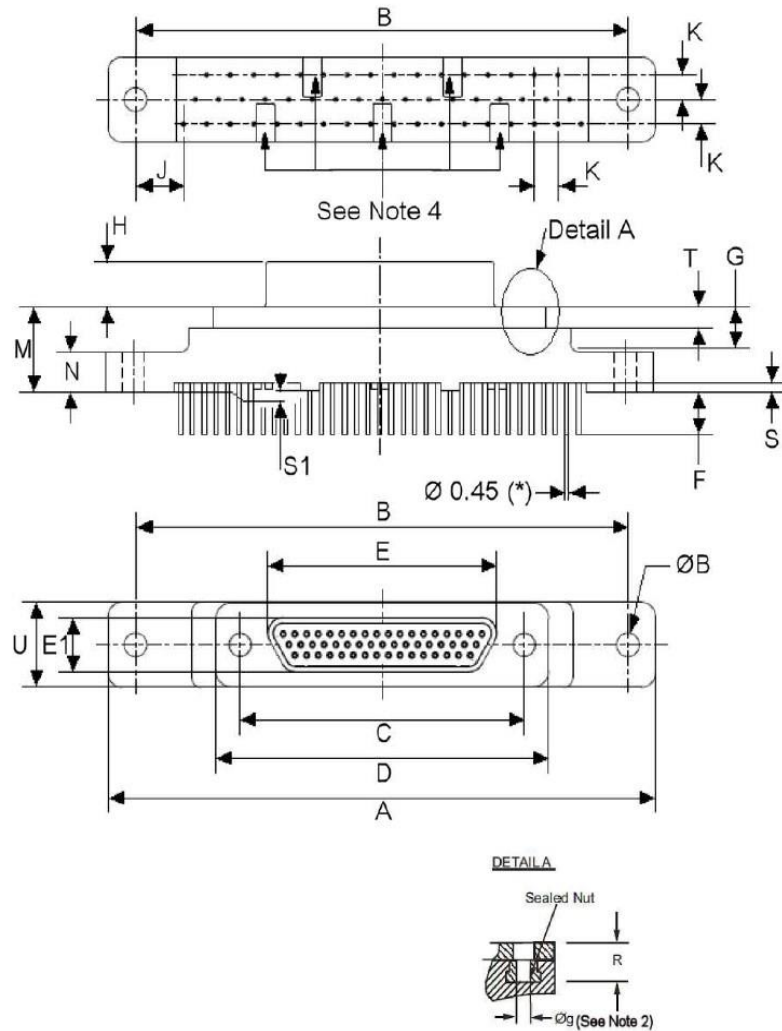
FIGURE 2.2I - CONNECTORS TYPE - FR139
