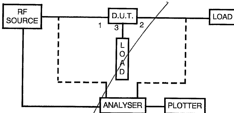
FIGURE IV - CIRCULATOR INSERTION LOSS TEST SET-UP
