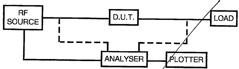
FIGURE I - ISOLATOR ISOLATION AND INSERTION LOSS TEST SET-UP
