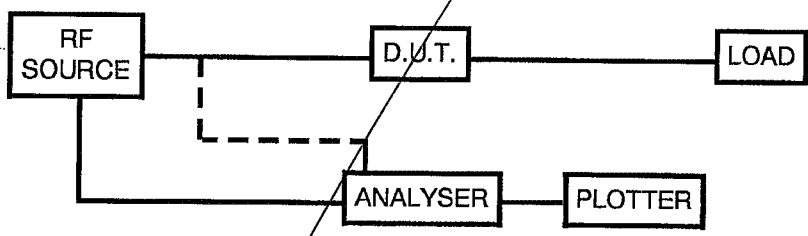
FIGURE III - CIRCULATOR ISOLATION TEST SET-UP
