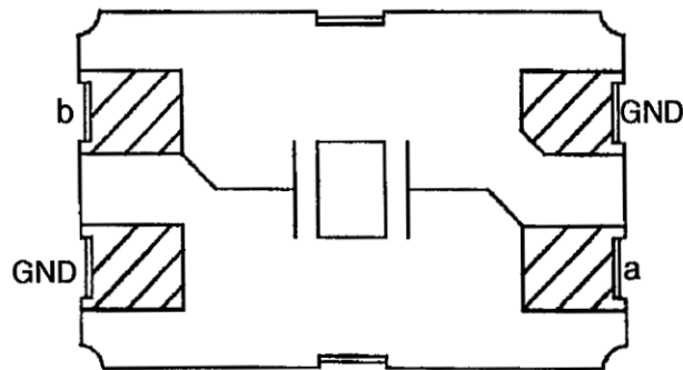
FIGURE 3 - FUNCTIONAL DIAGRAM
