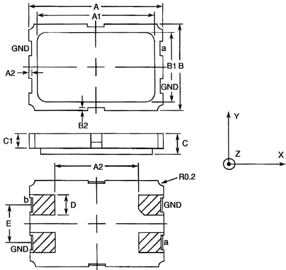
FIGURE 2 - PHYSICAL DIMENSIONS
