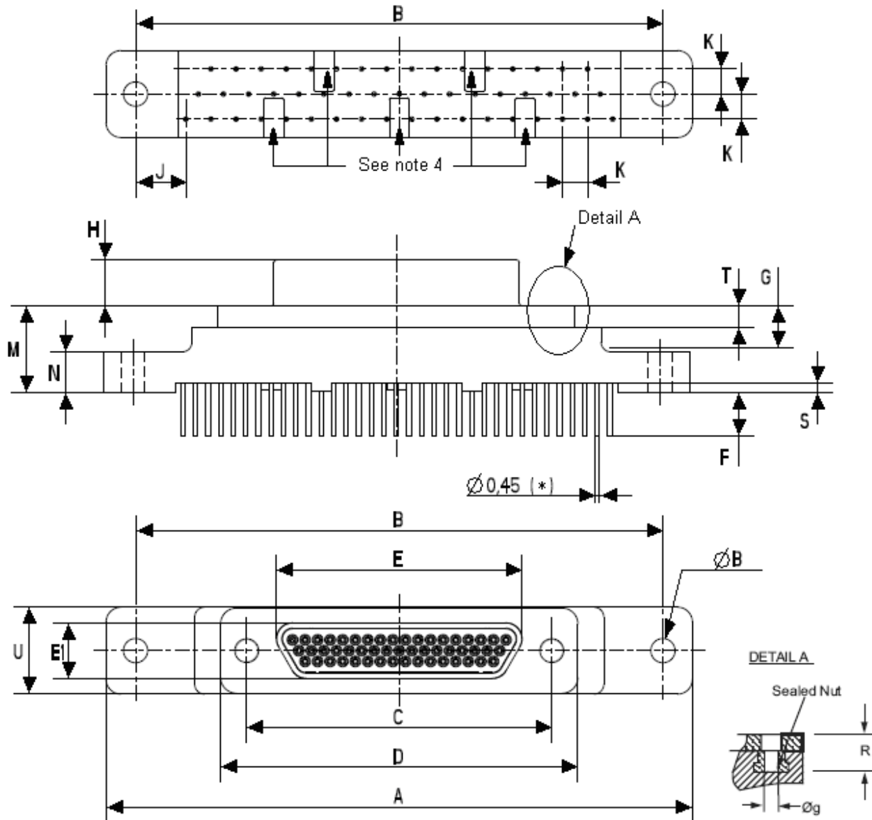
FIGURE 2.2J - CONNECTORS TYPE - FR139 RECEPTACLE FEMALE CONTACTS - SIZE 51
